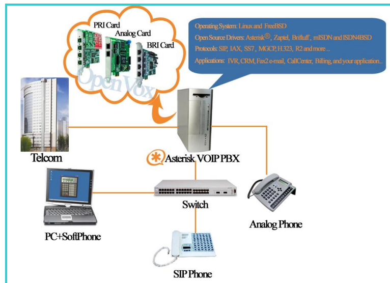
Figure 1: Asterisk Setup
